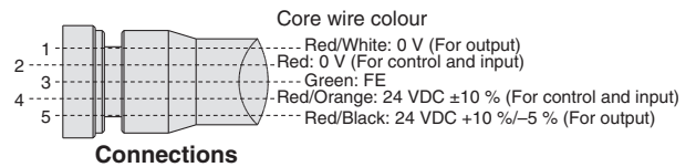
Socket pin arrangement
