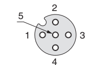
Socket connector pin arrangement A-coded (Normal key)
