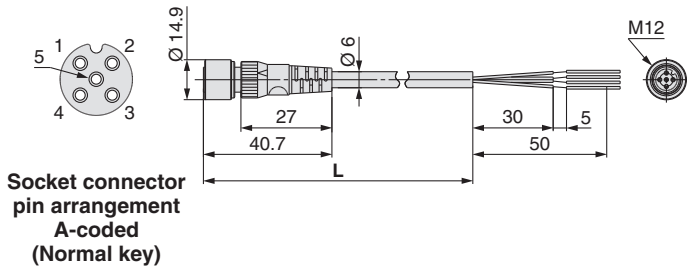
Socket connector pin arrangement A-coded (Normal key)
