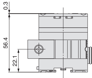
EX600-DX□C
