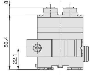
EX600-DX□D
