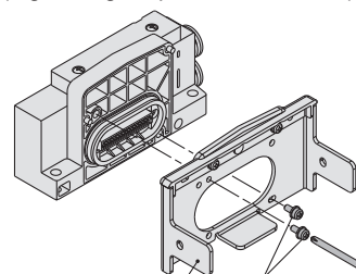
Valve plate Valve holding screw
