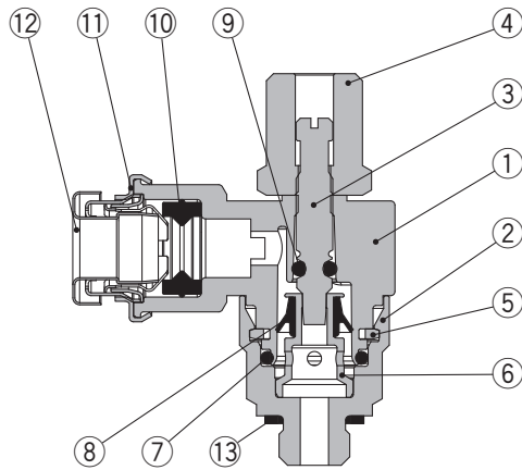
Meter-out
