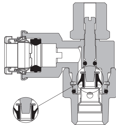
Meter-in
