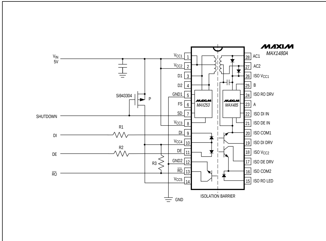
Figure 3. MAX1480A Low-Power Shutdown Mode
